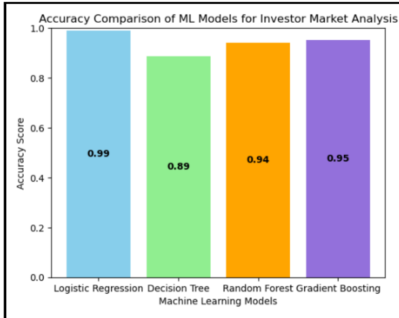
Fig. 14: Accuracy Comparison of Machine Learning Models
