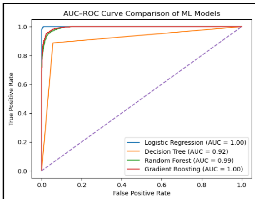
Fig. 15: AUC-ROC Curve Comparison of Machine Learning Models
